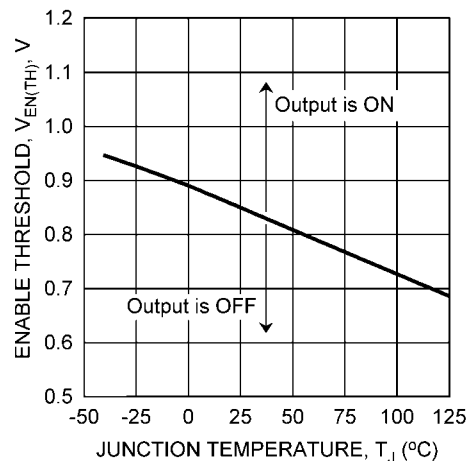
FIGURE 2. Enable Threshold
